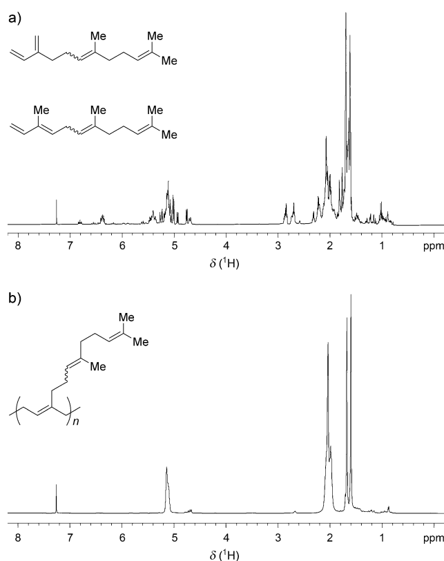
Figure 1. Selective polymerization of β-farnesene. The commercially available mixture can be used (a), only the β isomer is polymerized (b). For details see the Supporting Information.
