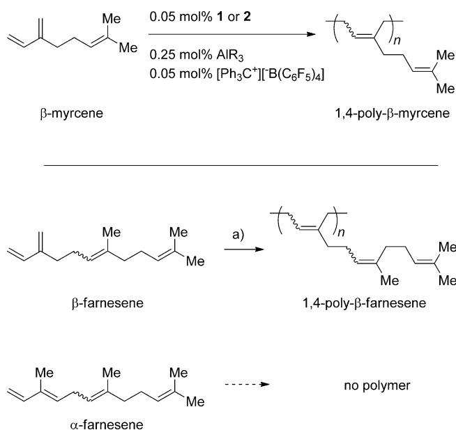
Scheme 2. Selective polymerizations of β-myrcene and β-farnesene using precatalysts 1 or 2 . a) 0.05 mol% 1 or 2 , 1.5 mol% AlR 3 (alkylating + drying agent), 0.05 mol% [Ph 3 C] + [B(C 6 F 5 ) 4 ] − . Because farnesene was used as obtained, a larger amount of trialkylaluminum reagent was used; it served as a drying agent as well as an alkylation reagent.
